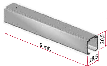
art. 2201 Binario in alluminio Aluminium rail
