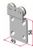
art. 3322 Carrello superiore esterno, con 2 cuscinetti a sfere External upper truck with 2 roller bearing
