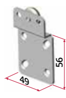
art. 3302 Carrello superiore esterno, con 1 cuscinetto a sfere External upper truck with 1 roller bearing
