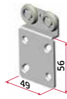
art. 3311 Carrello superiore interno, con 2 cuscinetti a sfere Internal upper truck with 2 roller bearing
