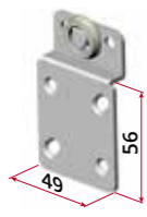
art. 3301 Carrello superiore interno, con 1 cuscinetto a sfere Internal upper truck with 1 roller bearing
