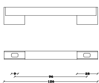
ART. 114 MANIGLIA IN CUOIO HIDE HANDLE
