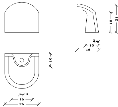
ART. 104 MANIGLIA IN CUOIO / HIDE HANDLE
