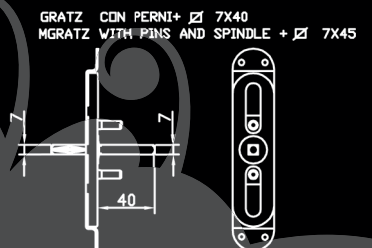
Mec. Cremonese 4F-CCCE-08
