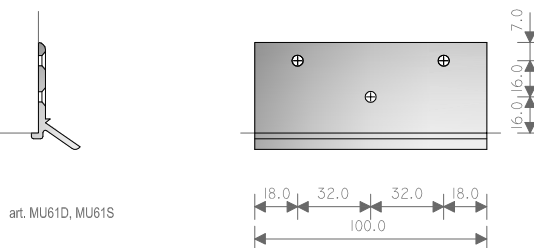
Internal lower slider H33
