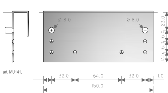
Interno upper truck H70
