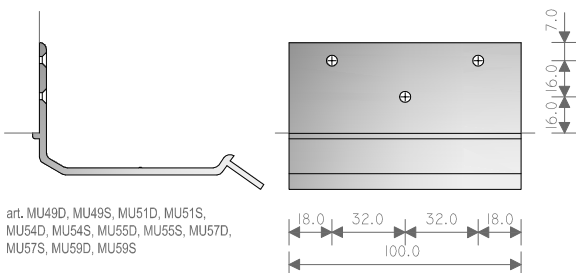
External lower slider H33
