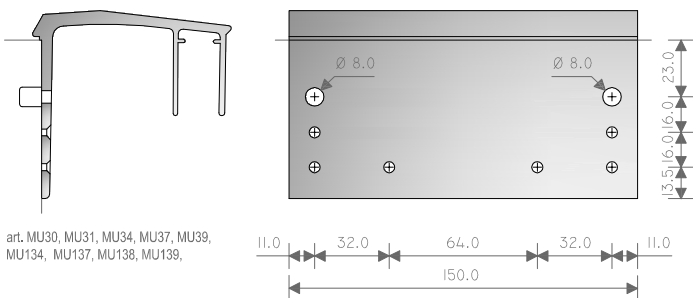
External upper truck H70
