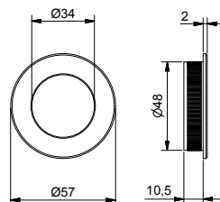
FORATURA PORTA DOOR DRILLING
